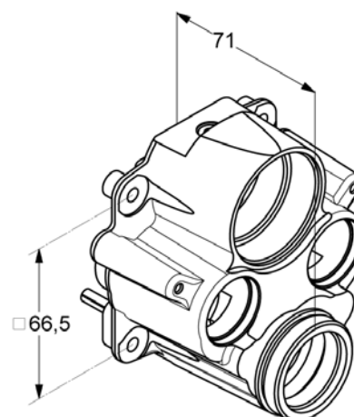
Dimensional drawing
