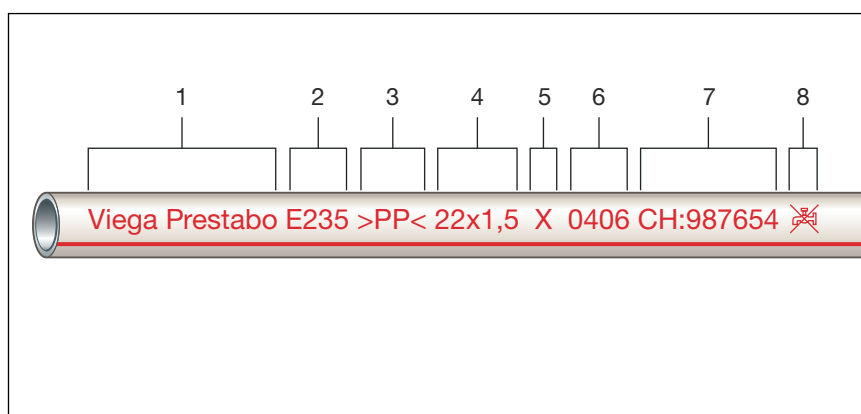
Abb. 7: Rohr PP-ummantelt
