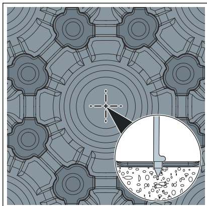
Abb. 2: Fonterra Base-Noppenplatte 12/15
